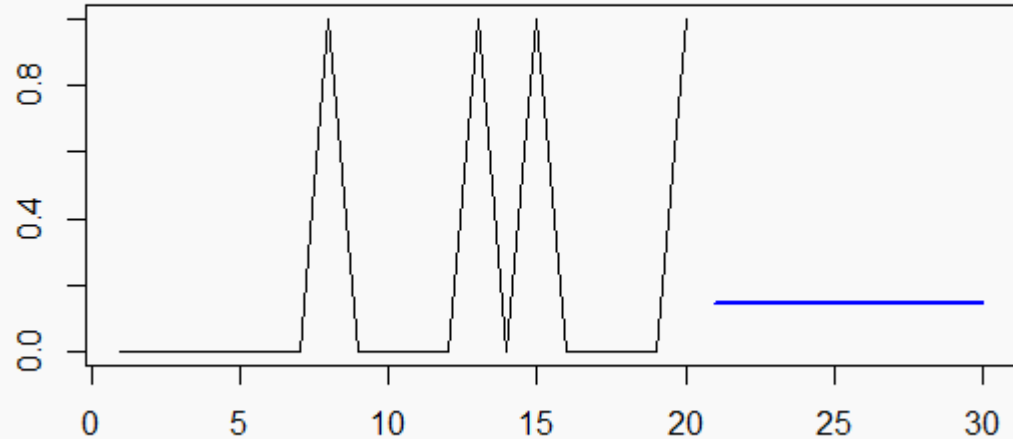
Forecasts from Croston's method
