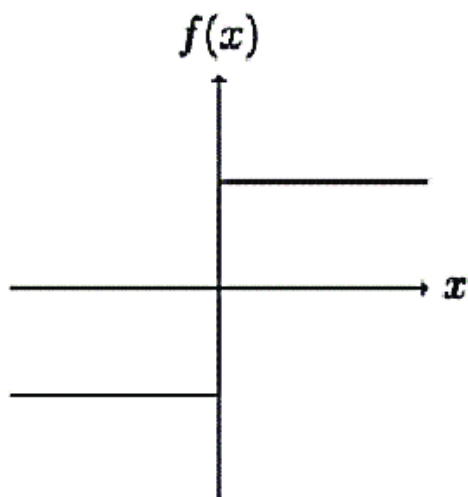
lump function
